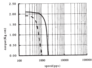
MODEL :H39Y384001 TORQUE VS. SPEED CURVE DRIVER : DUAL CHOPPER SUPPLY VOLTAGE : 24V CURRENT: 0.5A
