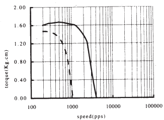
MODEL :H39Y346001 TORQUE VS. SPEED CURVE DRIVER : DUAL CHOPPER SUPPLY VOLTAGE : 24V CURRENT: 0.3A
