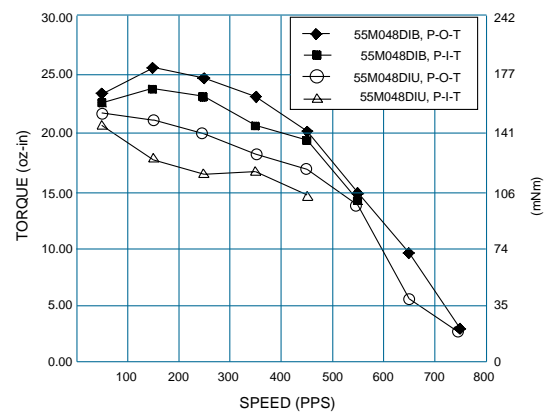
TORQUE-SPEED CURVE*
