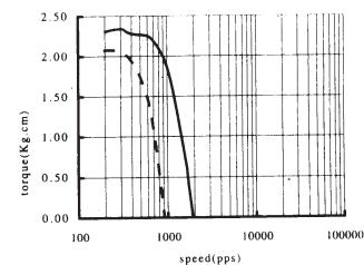
MODEL :H39Y204001 TORQUE VS. SPEED CURVE DRIVER : DUAL CHOPPER SUPPLY VOLTAGE : 24V CURRENT: 0.4A
