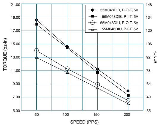
TORQUE-SPEED CURVE*
