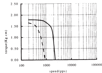
MODEL :H39Y206001 TORQUE VS. SPEED CURVE DRIVER : DUAL CHOPPER SUPPLY VOLTAGE : 24V CURRENT: 0.5A
