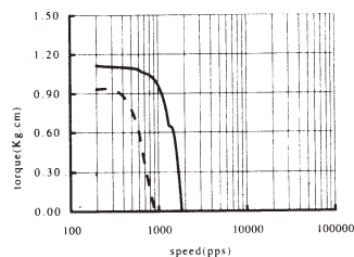
MODEL :H39Y386001 TORQUE VS. SPEED CURVE DRIVER : DUAL CHOPPER SUPPLY VOLTAGE : 24V CURRENT: 0.8A
