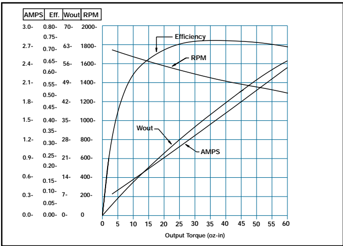
Motor Performance at 100% PWM
