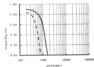
MODEL :H39Y444001 TORQUE VS. SPEED CURVE DRIVER : DUAL CHOPPER SUPPLY VOLTAGE : 24V CURRENT: 0.3A
