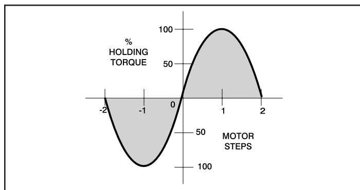
Figure 4: Torque Deflection.
