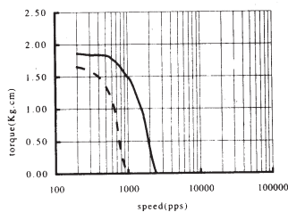
MODEL :H39Y346002 TORQUE VS. SPEED CURVE DRIVER : DUAL CHOPPER SUPPLY VOLTAGE : 24V CURRENT: 0.16A
