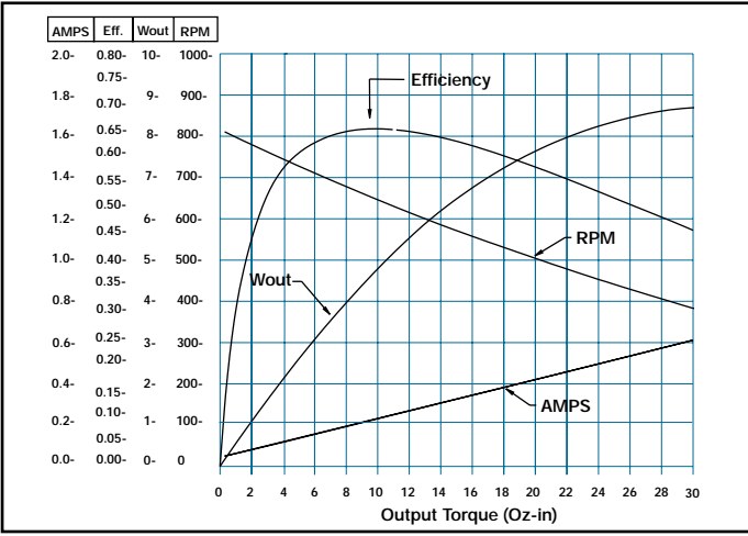
Motor Performance at 50% PWM
