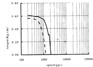
MODEL :H39Y204001 TORQUE VS. SPEED CURVE DRIVER : DUAL CHOPPER SUPPLY VOLTAGE : 24V CURRENT: 0.4A
